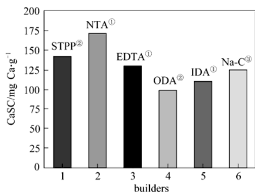
Figure 7 Calcium-sequestering capacities (CaSC) of different organic builders
