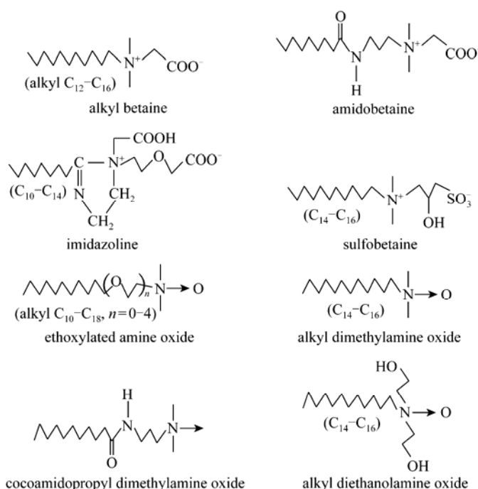
Figure 5 Structures of some major zwitterionic surfactants in detergent compositions
