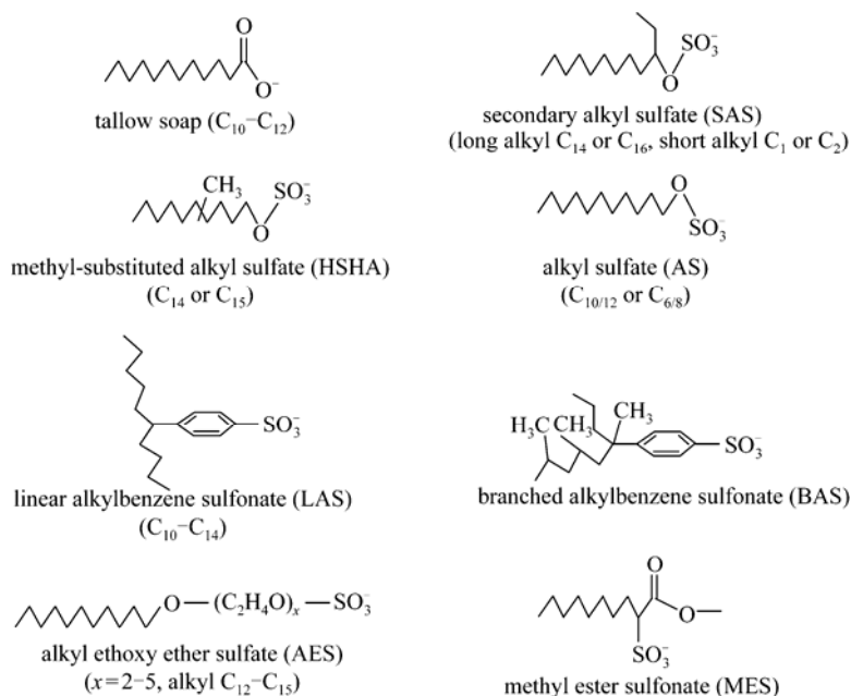
Figure 1 Structures of some major anionic surfactants in detergent compositions
