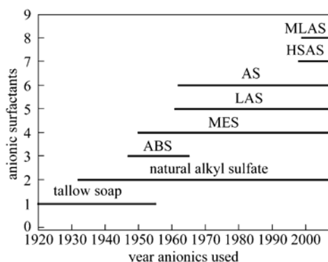
Figure 2 Evolution of some major anionic surfactants [3] HSAS—highly soluble alcohol sulfate; MLAS—modified linear alkyl benzene sulfonate
