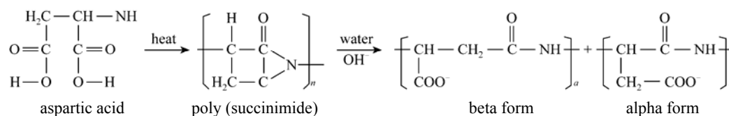
Figure 9 Synthesis process of the thermal poly(aspartic acid)
