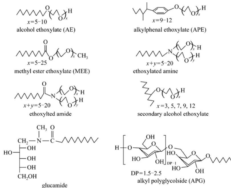
Figure 3 Structures of some major nonionic surfactants in detergent compositions
