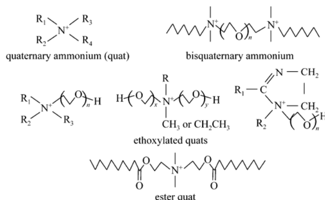
Figure 4 Structures of major cationic surfactants in detergent compositions
