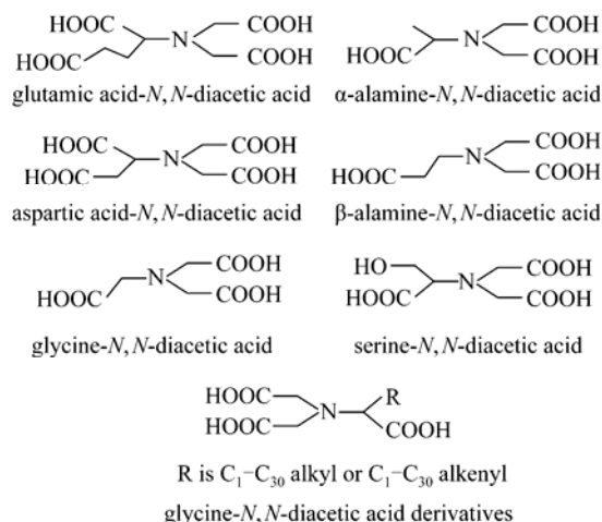
Figure 8 Amino acid- N,N -diacetic acid and derivatives
