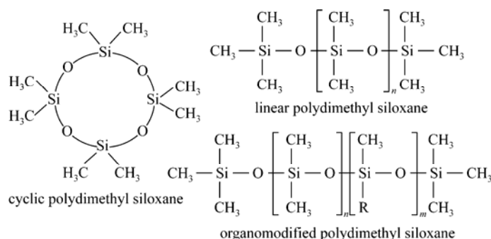
Figure 6 Structures of polydimethyl siloxanes and their derivatives
